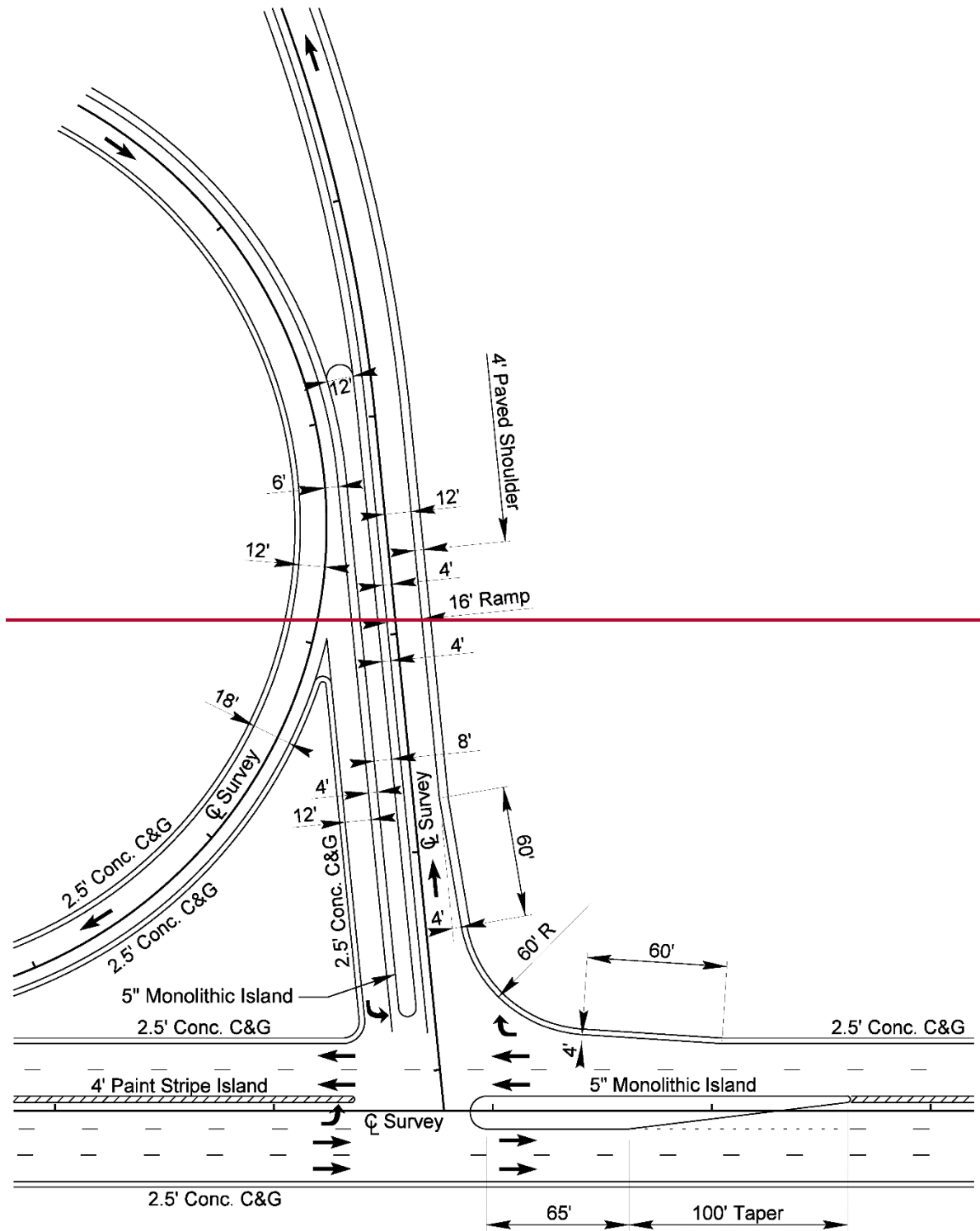
Figure 9-9 Plan for Loop Ramp Terminal Combination
