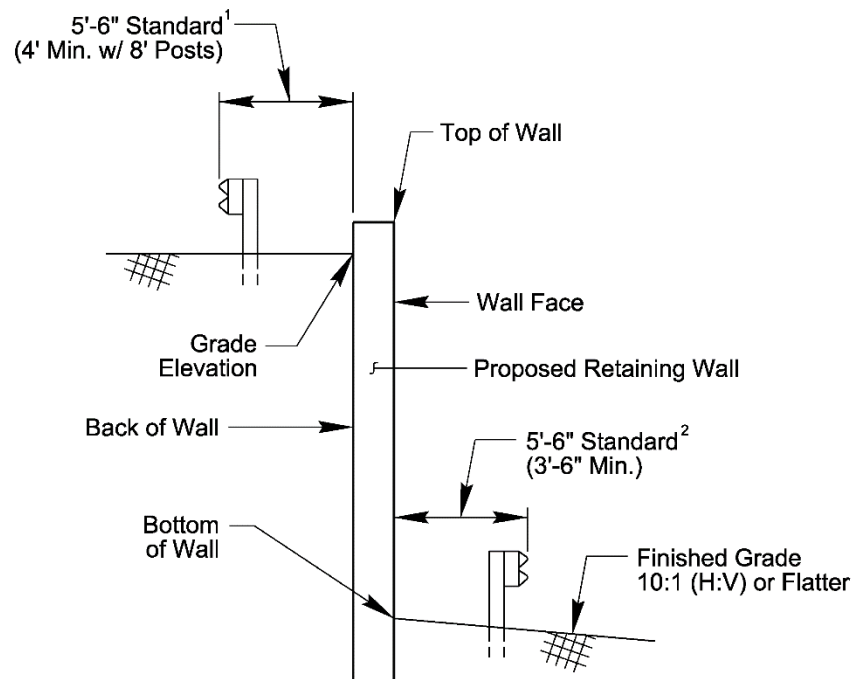
Figure 5-27 Offsets for Steel Beam Guardrail at Retaining Walls
