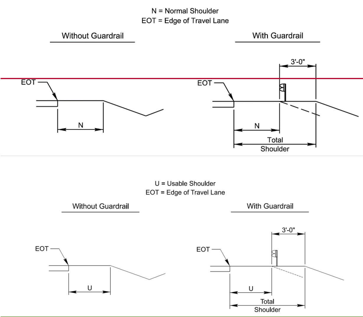
Figure 4-1 Usable and Total Shoulder Width for Locals and Collectors
