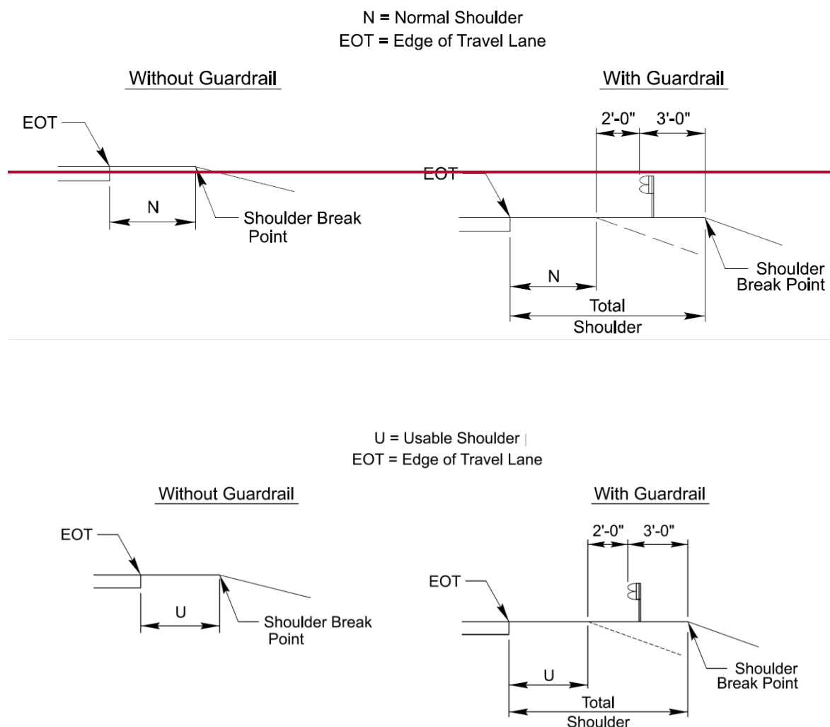
Figure 4-2 Usable and Total Shoulder Width for Arterials, Interstates, and Freeways
